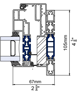
Awning & Casement (Concealed hinges)
