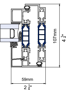
Door & Casement (Heavy solution, visible hinges)
