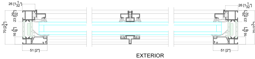
DETAIL 2
