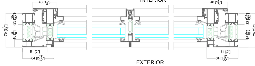
DETAIL 2
