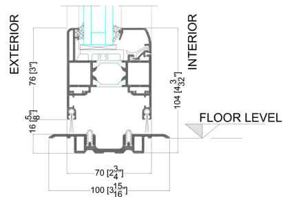
DETAIL 6.2
