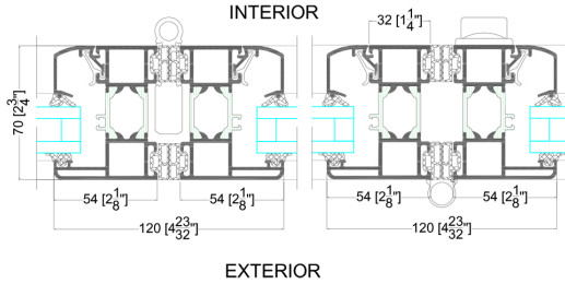
DETAIL 2
