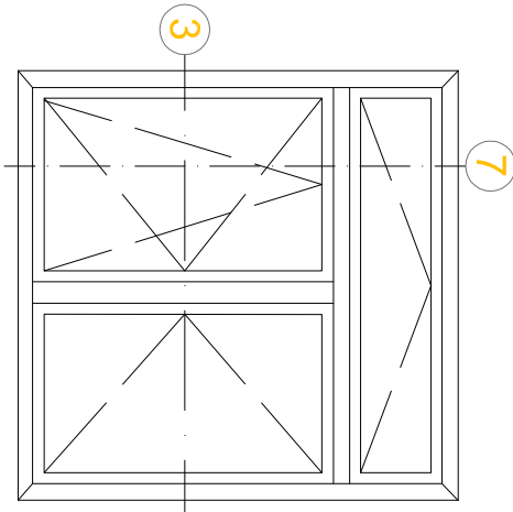
Double-vent window with toplight
