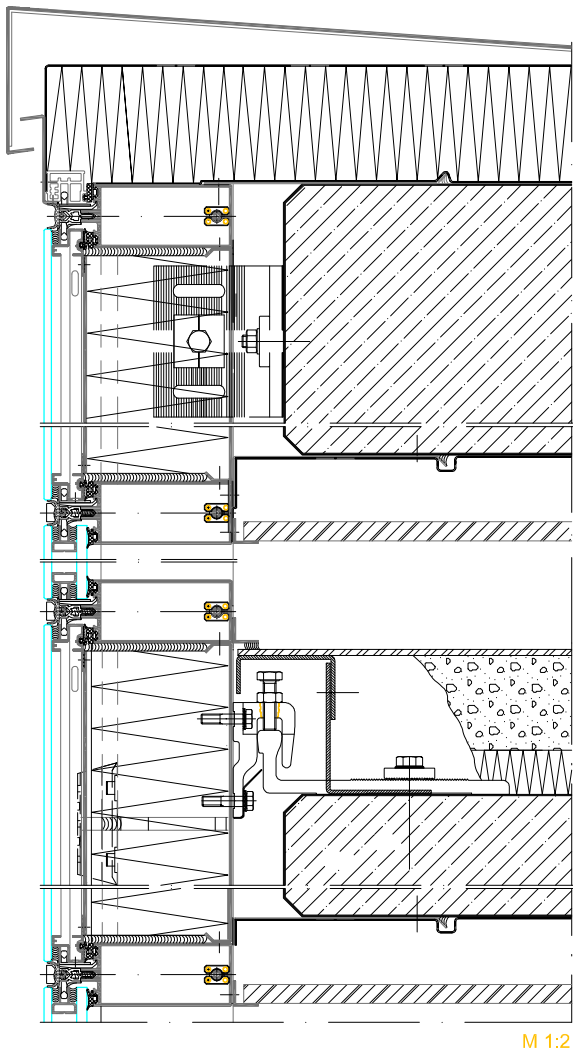
Fascia and intermediate floor attachments
