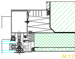
Flush-fitted dry glazing
