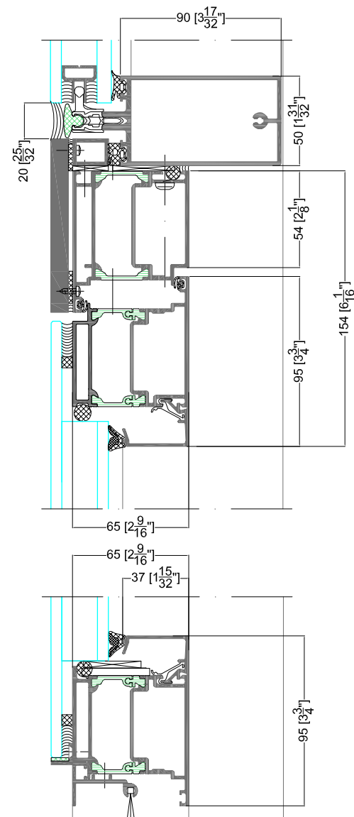
DETAIL 12 Wet sealing
