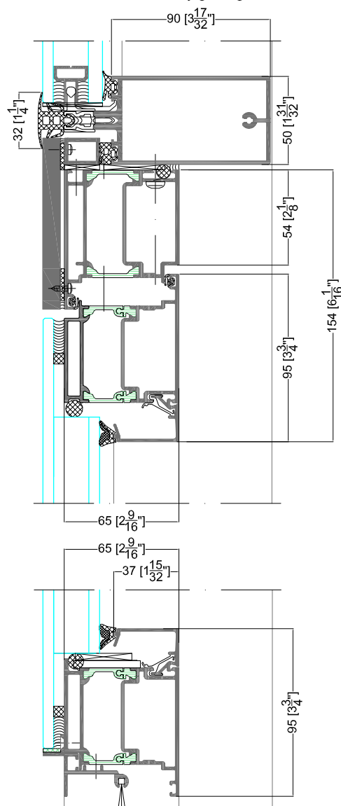
DETAIL 12 Flush-fitted dry glazing
