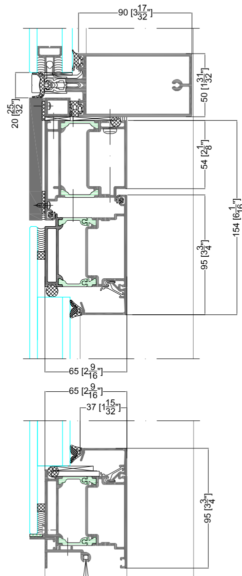
DETAIL 12 U-shaped dry glazing
