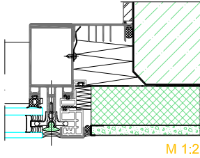
Wet sealing
