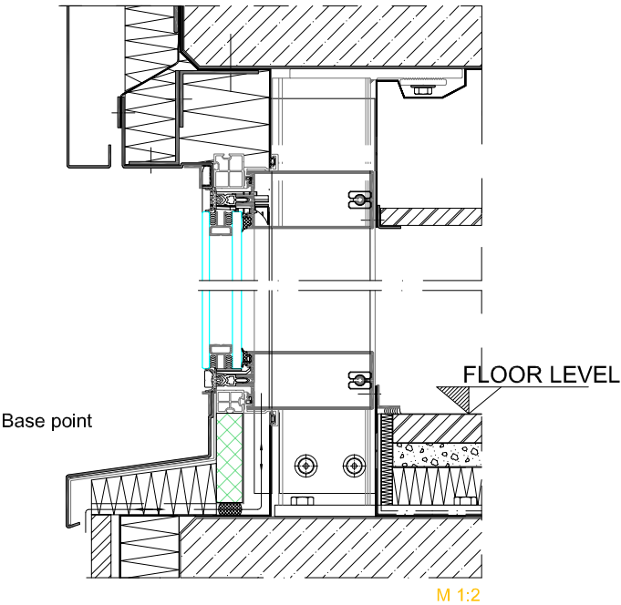
Attachment underneath the floor
