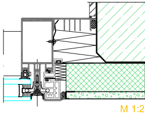
U-shaped dry glazing
