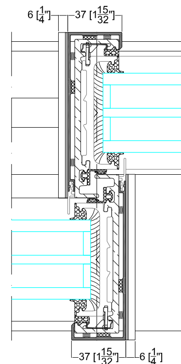
DETAIL 4
