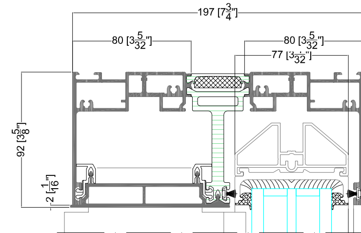
DETAIL 1.2
