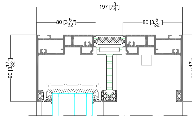
DETAIL 1.1
