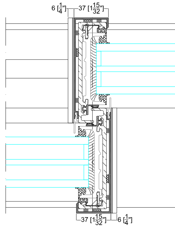
DETAIL 4
