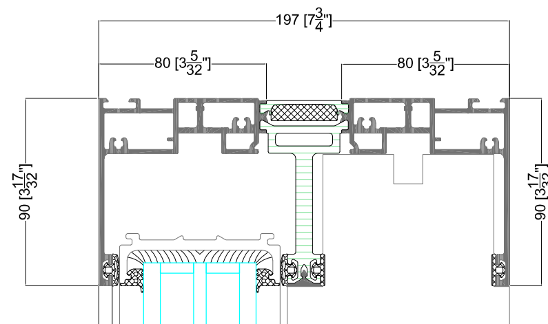
DETAIL 1.1
