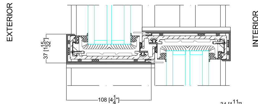
DETAIL 6/90
