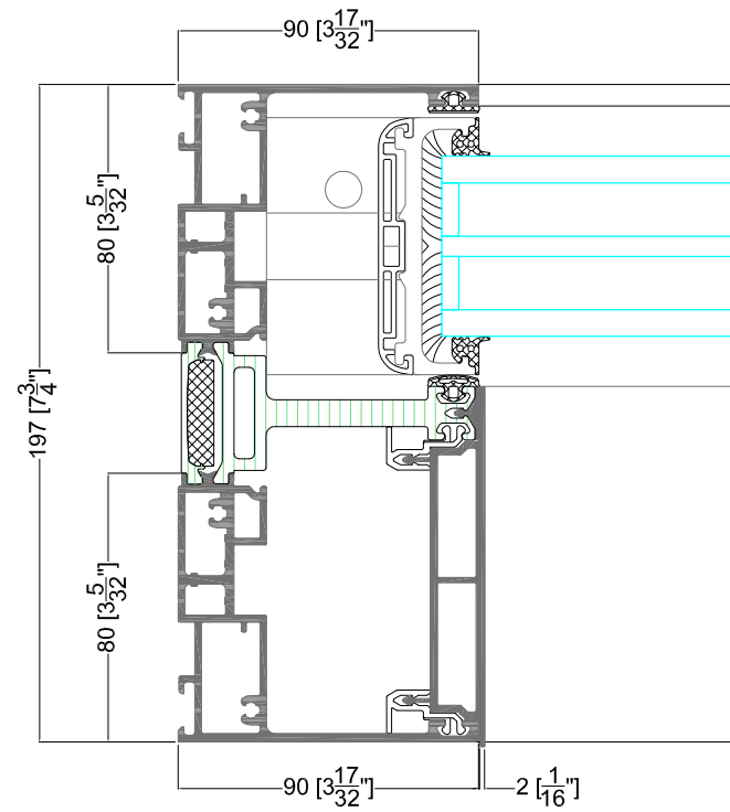
DETAIL 7.2
