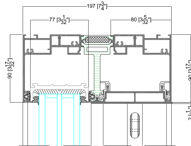
DETAIL 7.1
