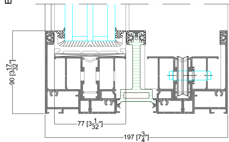
DETAIL 2.1
