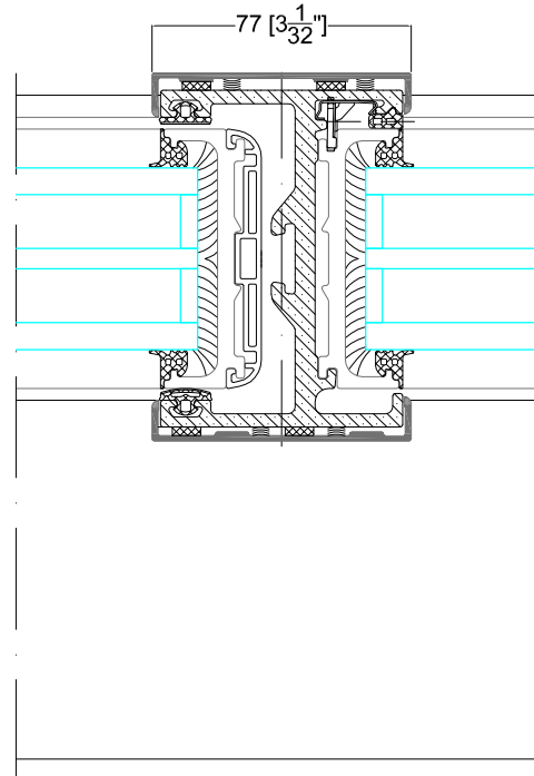
DETAIL 6 INTERIOR
