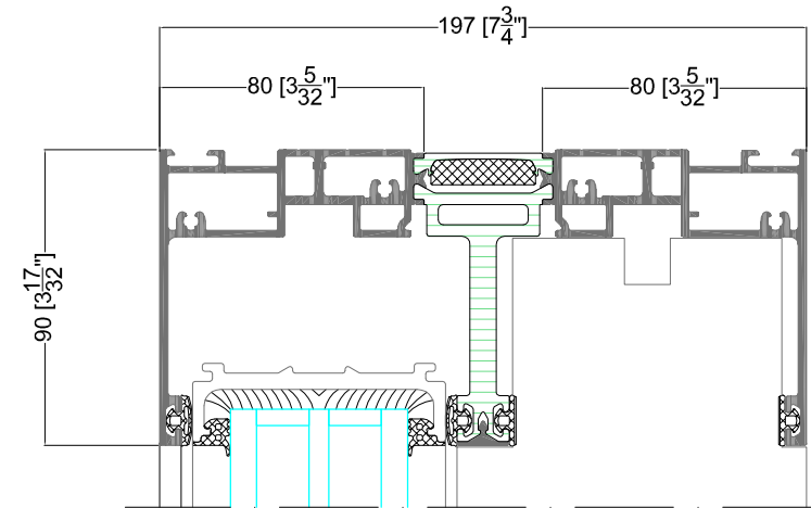
DETAIL 1.1
