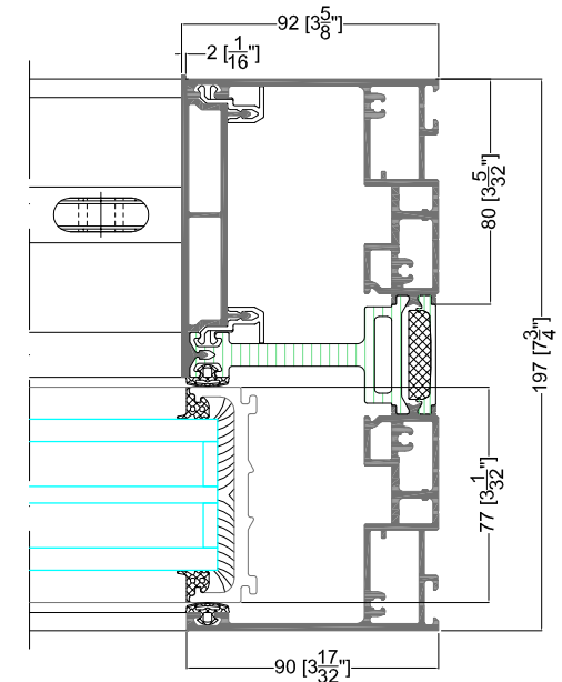
DETAIL 3.1
