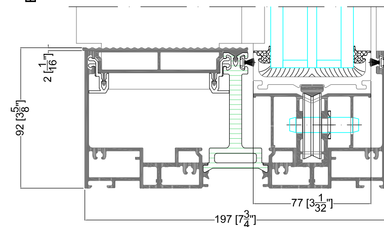
DETAIL 2.2
