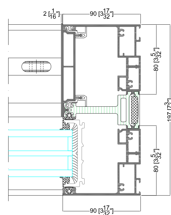
DETAIL 3.1
