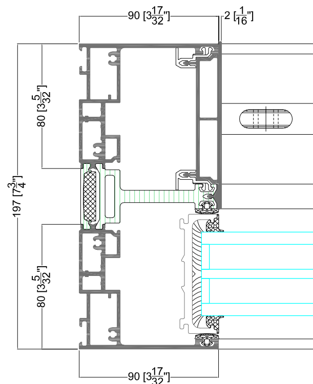
DETAIL 7.1
