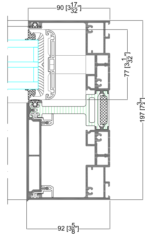
DETAIL 1.2
