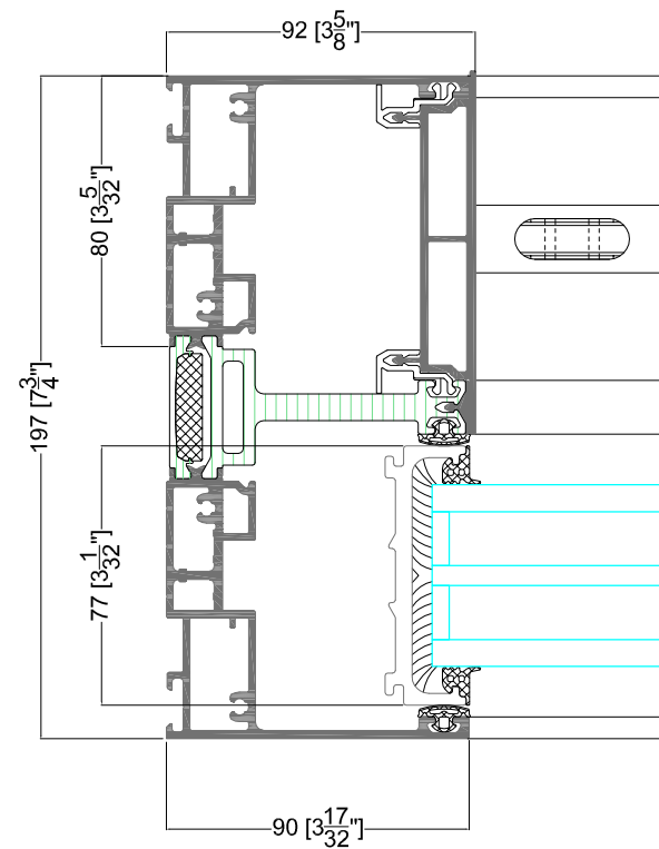
DETAIL 7.1
