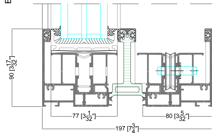
DETAIL 2.1
