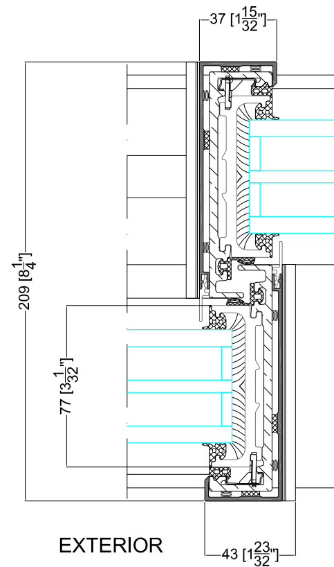
DETAIL 4
