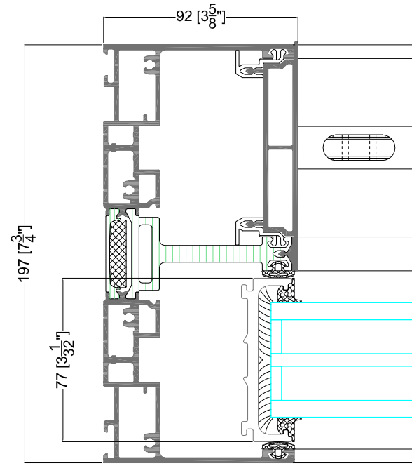
DETAIL 7.1
