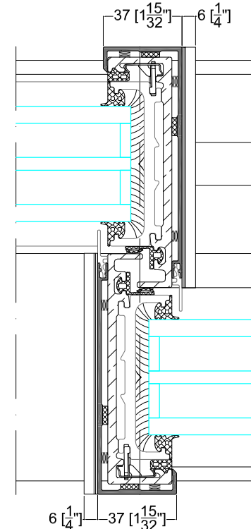
DETAIL 4
