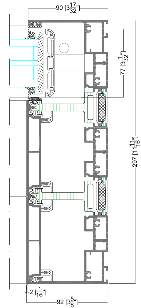
DETAIL 3.3
