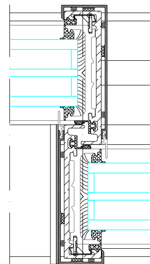
DETAIL 4
