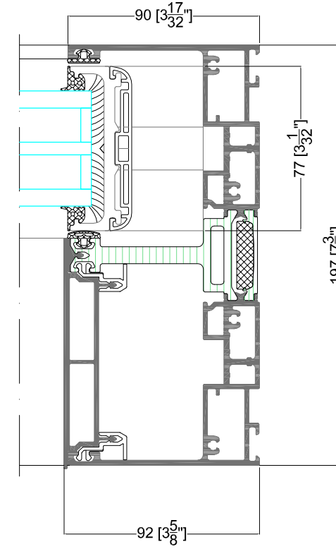
DETAIL 1.2
