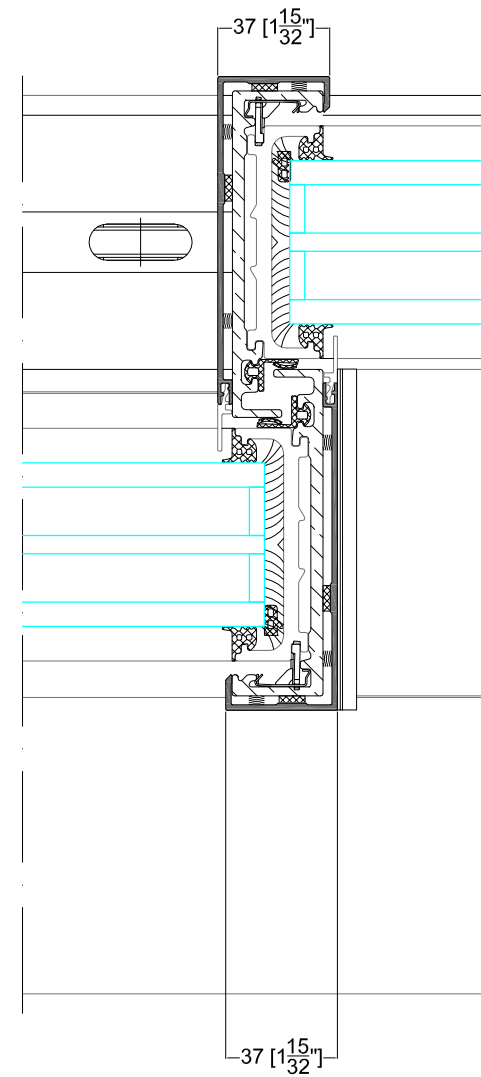
DETAIL 4
