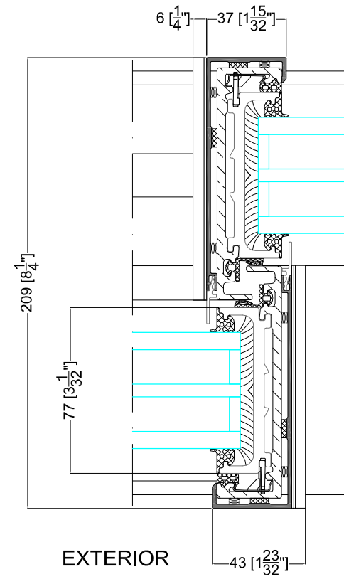
INTERIOR DETAIL 4
