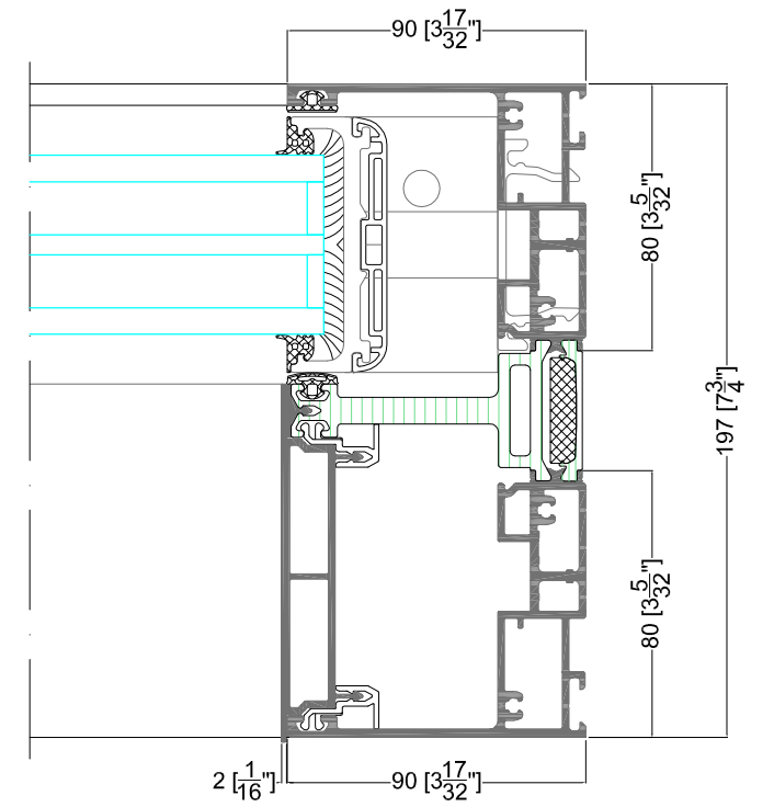
DETAIL 3.2
