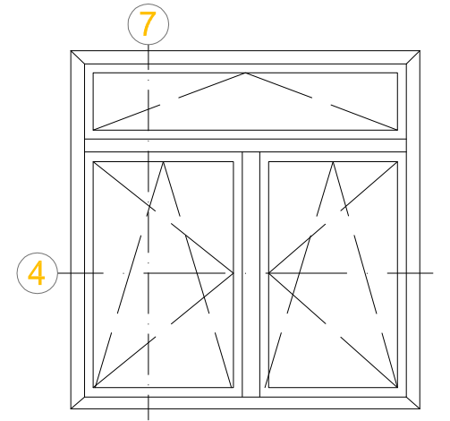
Vent + vent with toplight
