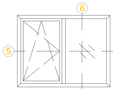
Single-vent window with fixed light
