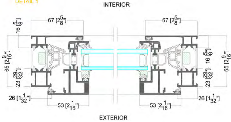
DETAIL 1
