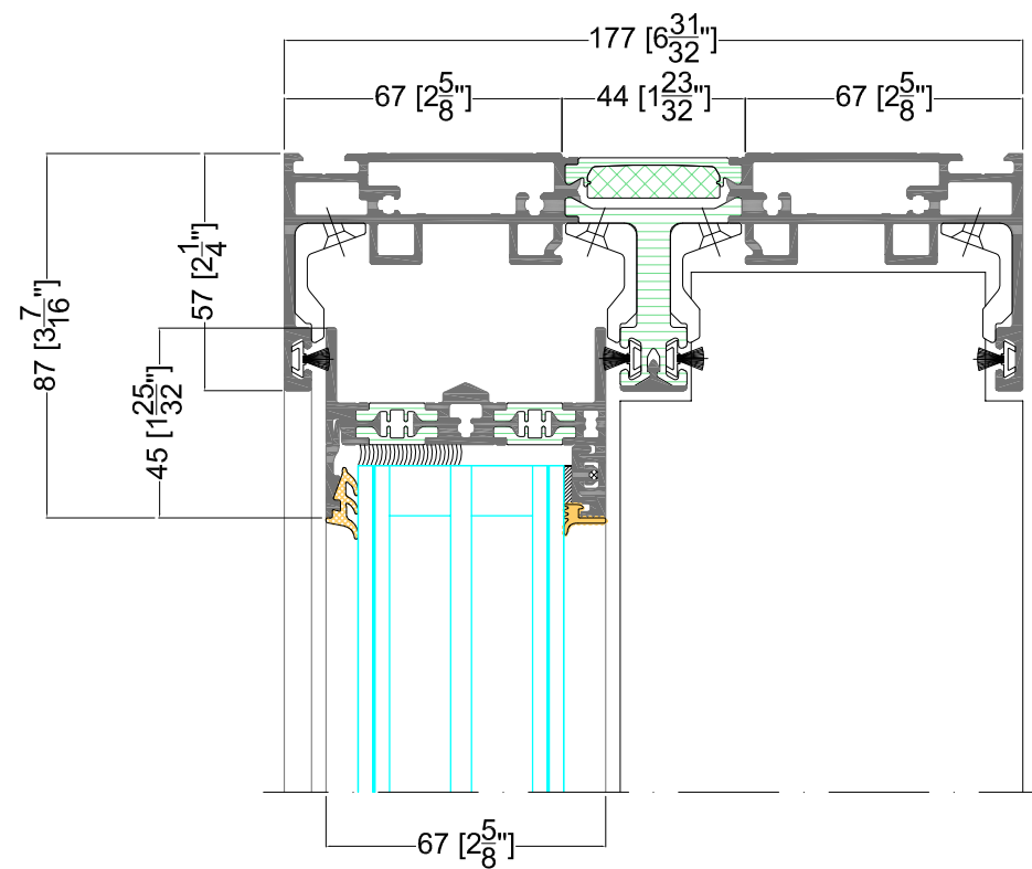
Top attachment 2A and 2A/1 left 57/57
