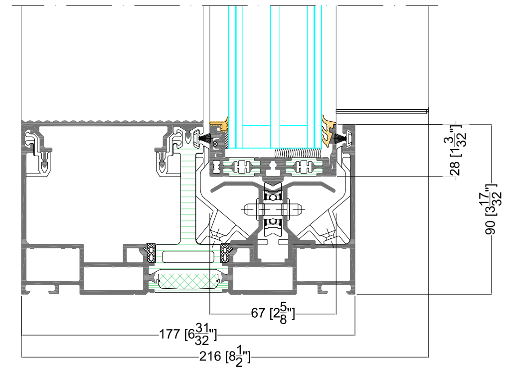
CONCEALED FRAME - GAP TRACK
