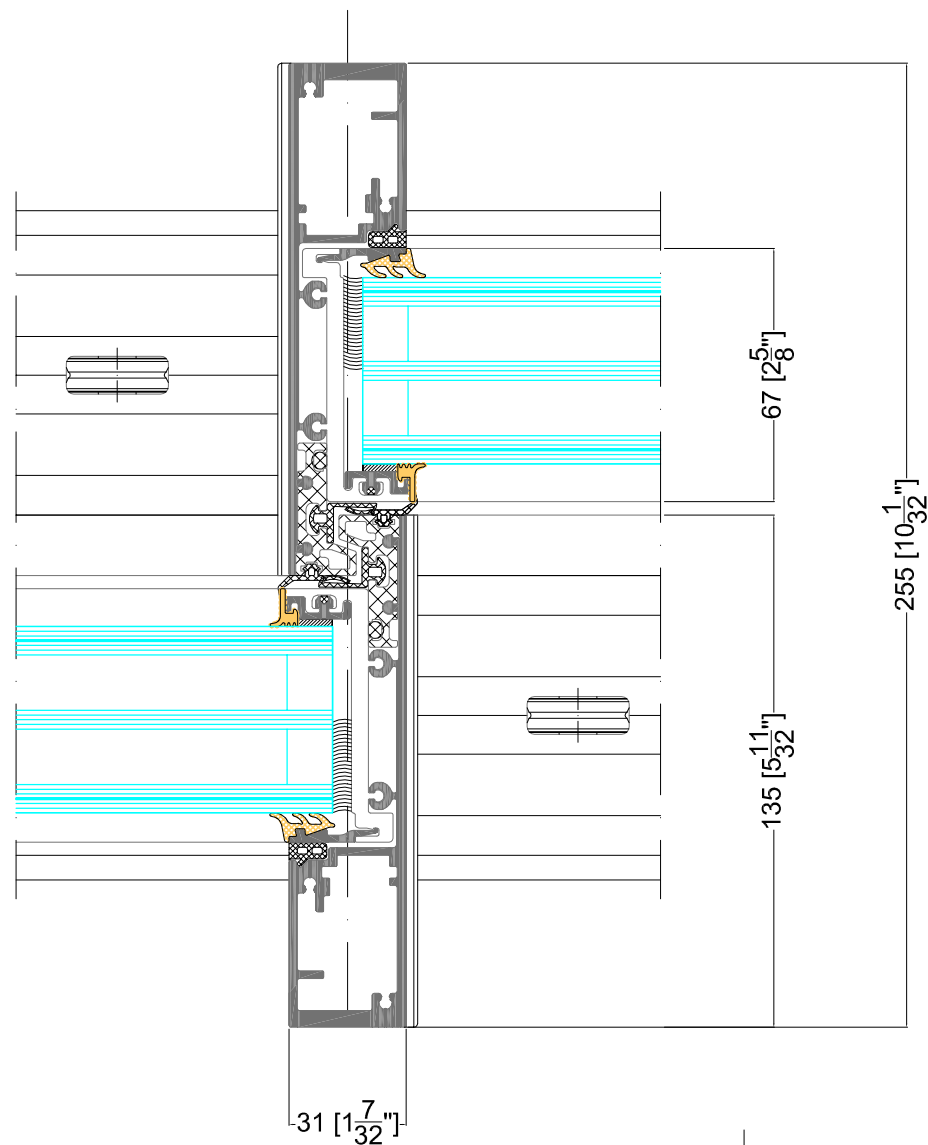
Centre connection 2A 57/57 and 90/90
