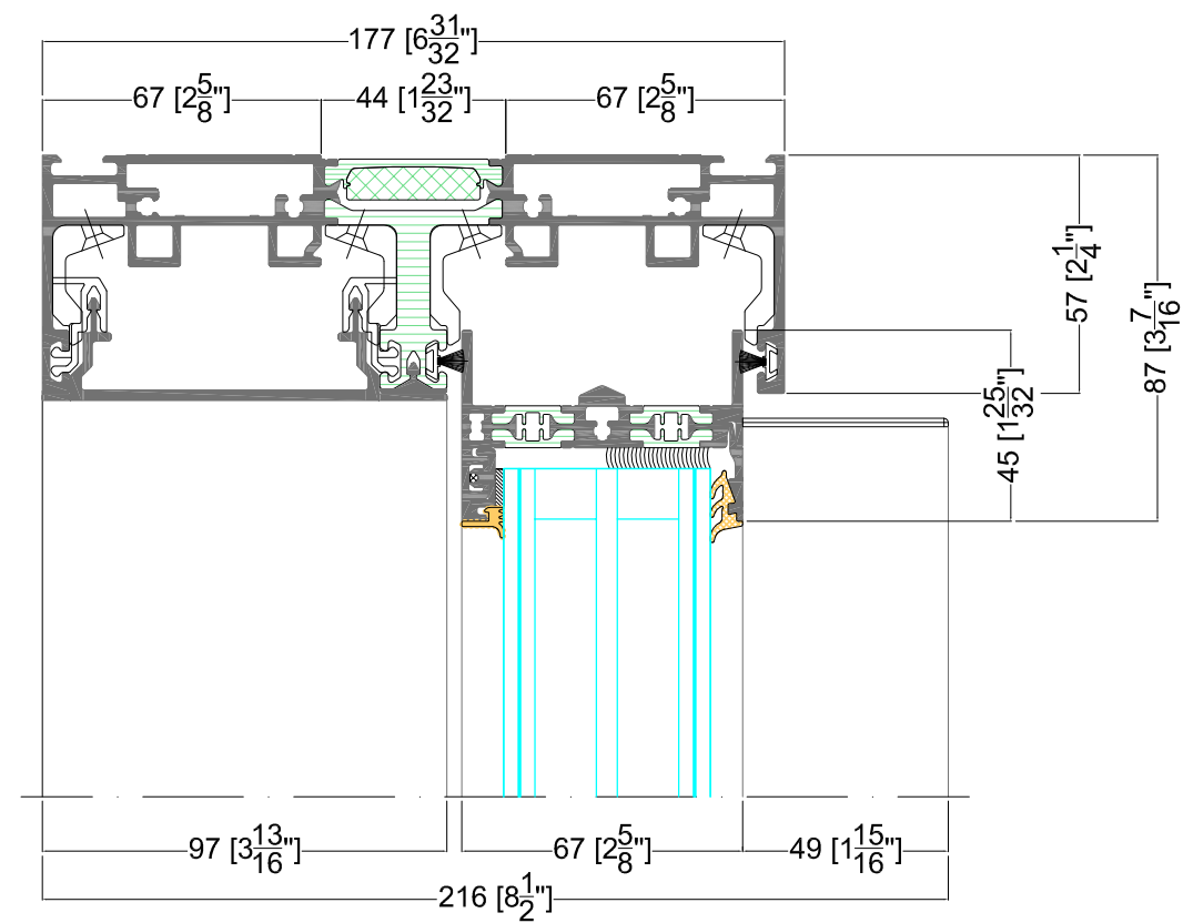
Top attachment 2A/1 right 57/57
