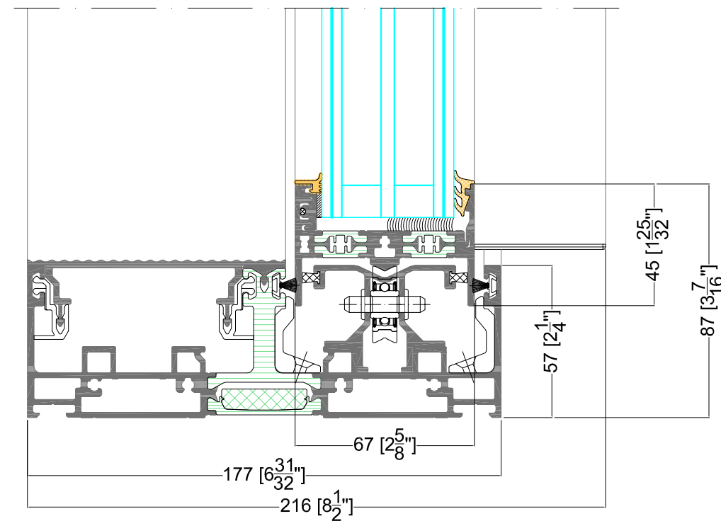
FLUSH TRACK - EXPOSED FRAME
