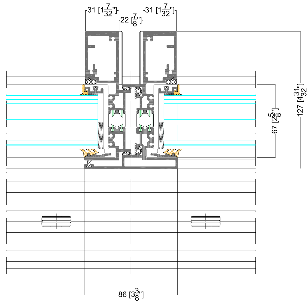
Centre attachment 2D all types
