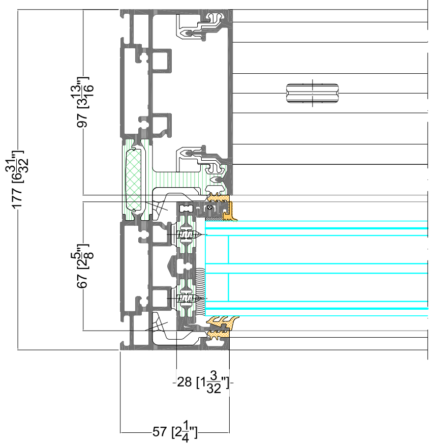
2A/1 left 57/57 light
