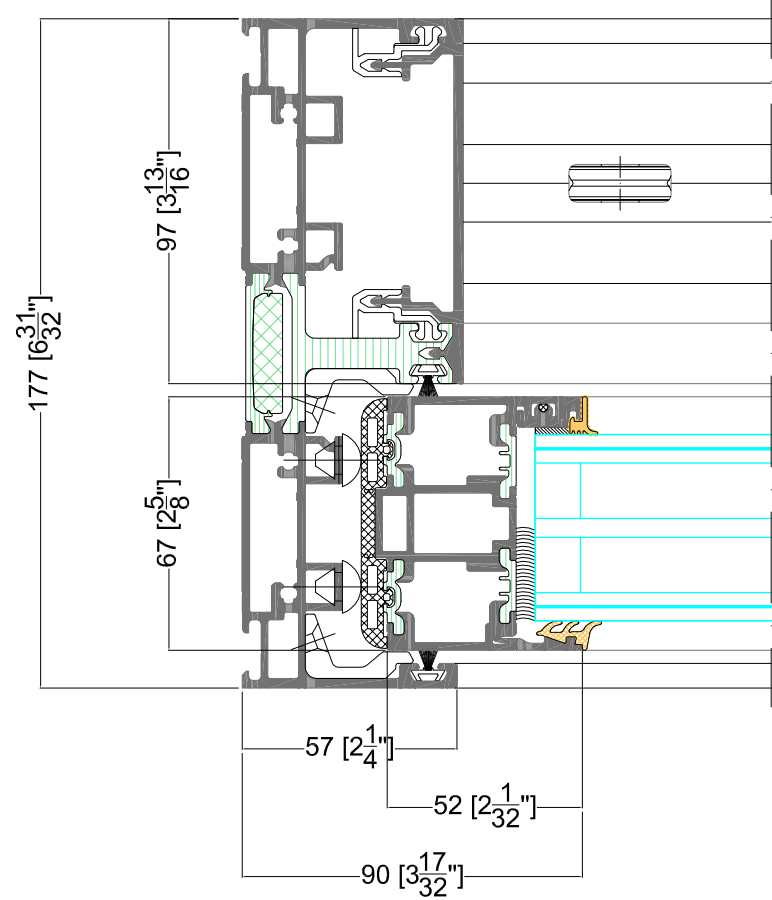
Left attachment 2A and 2A/1 57/57
