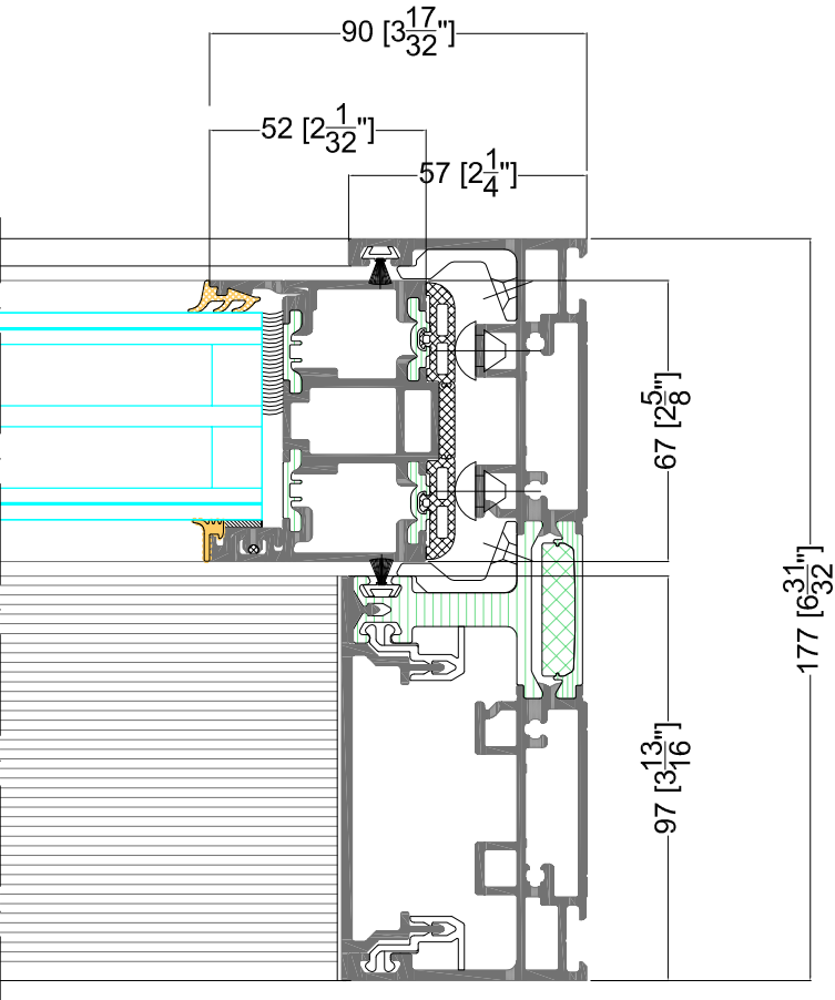
Right attachment 2A/1 57/57
