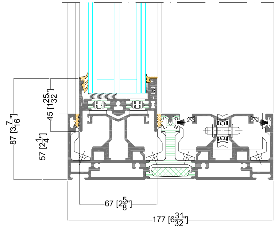
FLUSH TRACK - EXPOSED FRAME
