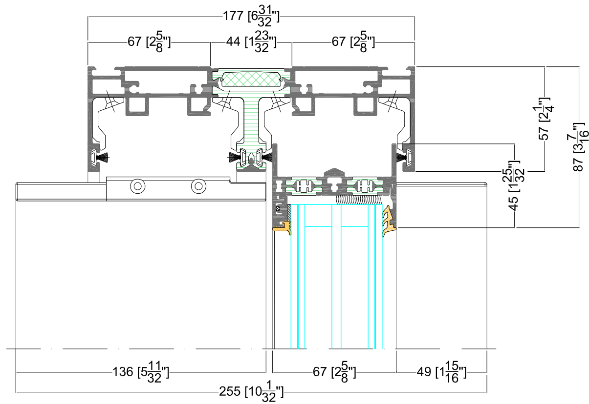
Top attachment 2A right 57/57
