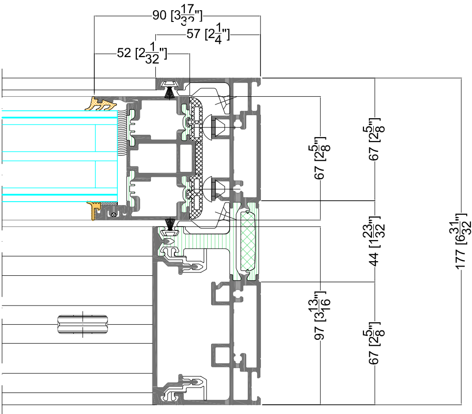
Right attachment 2A 57/57
