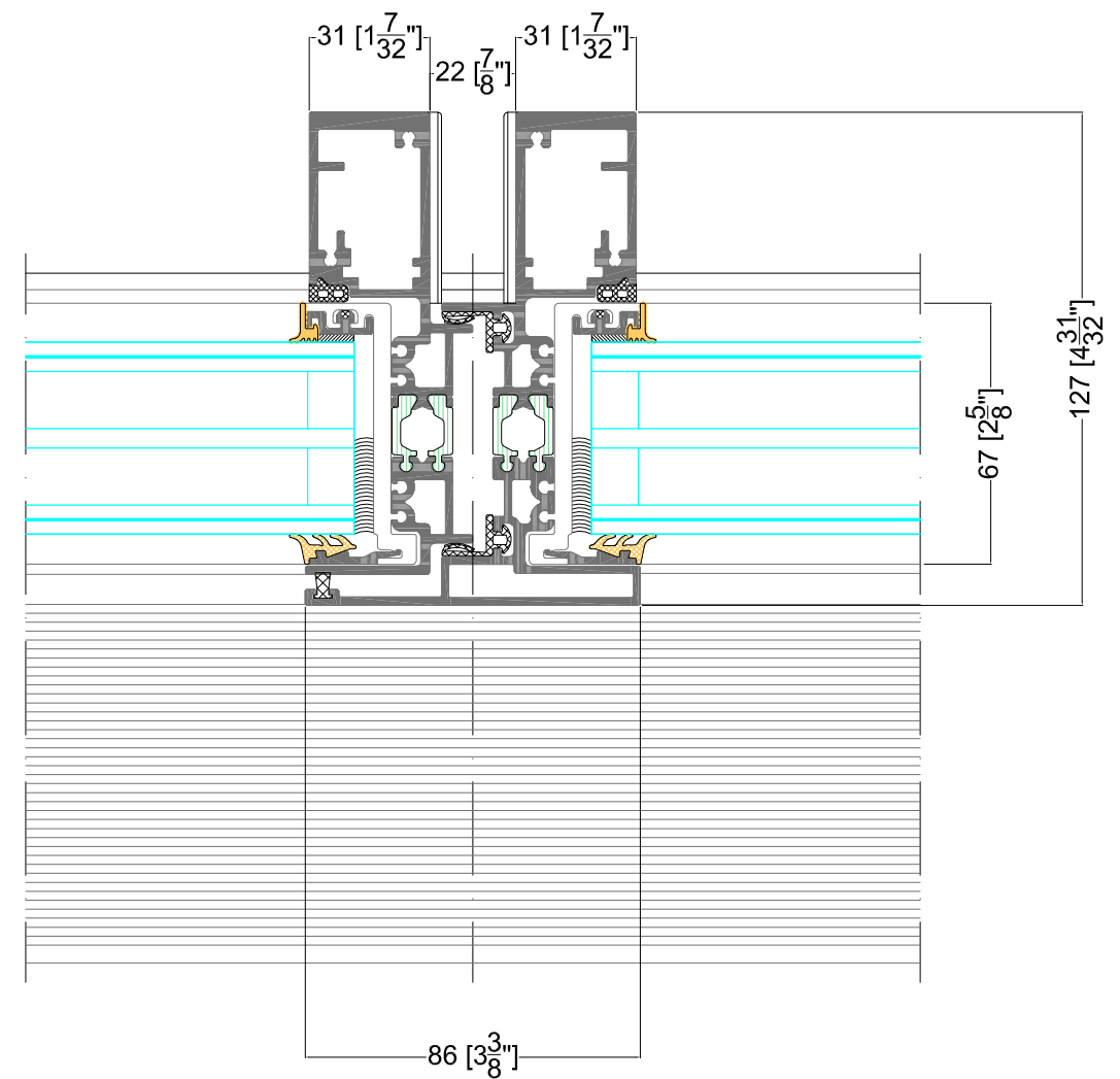
2D/1 all types
