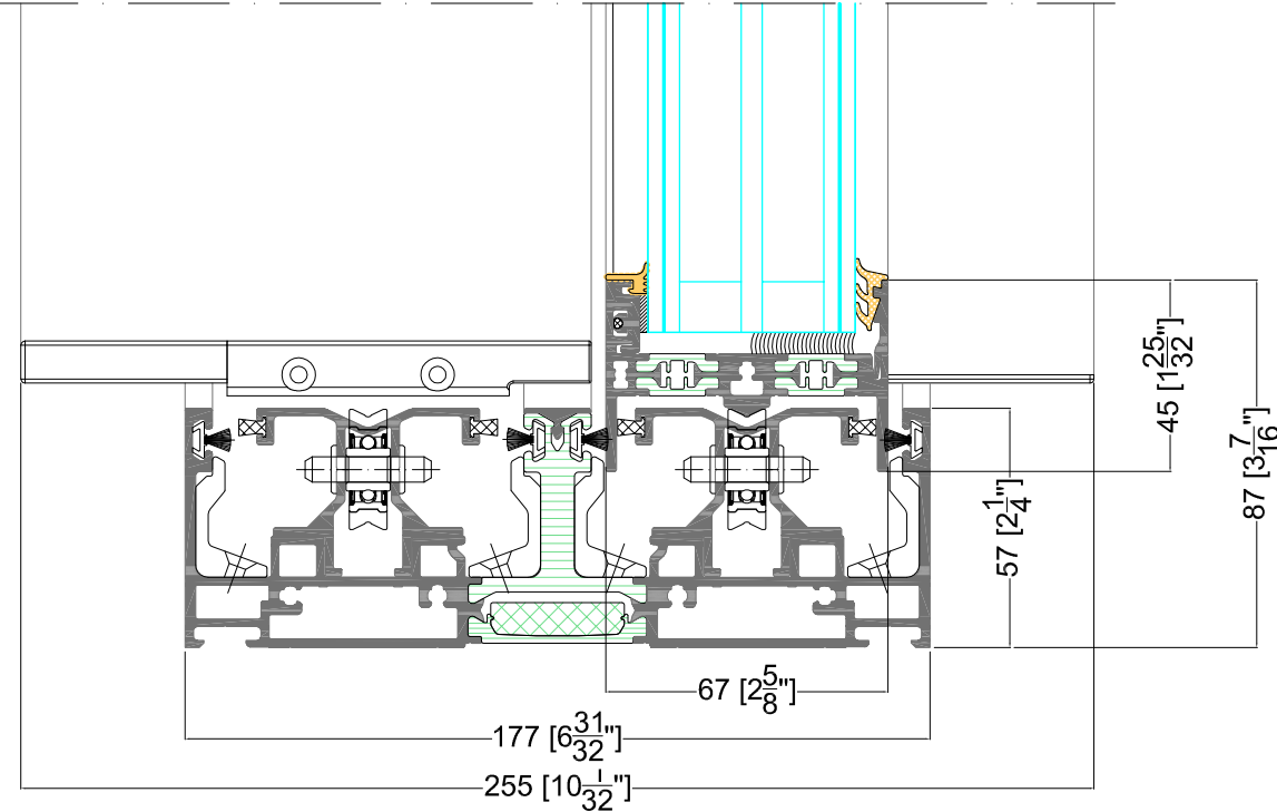
FLUSH TRACK - EXPOSED FRAME
