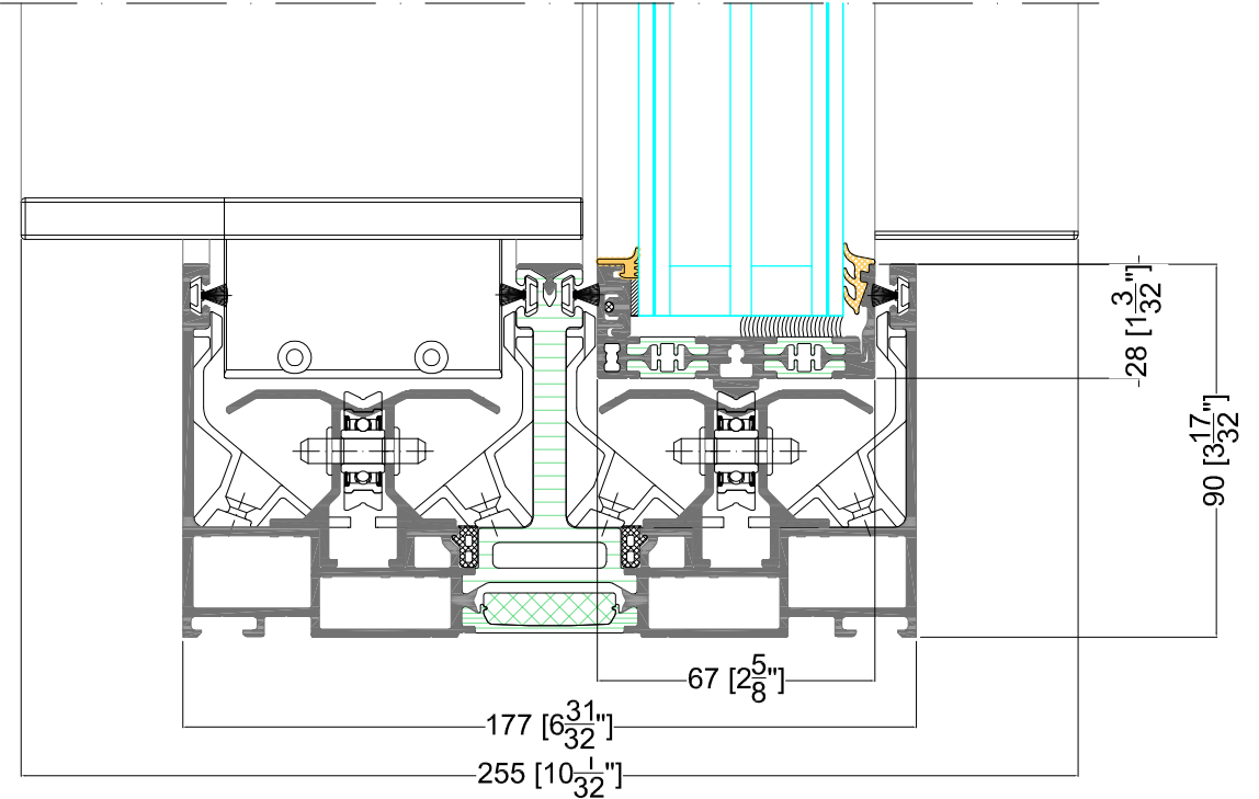
CONCEALED FRAME - GAP TRACK
