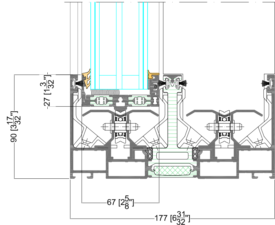
CONCEALED FRAME - GAP TRACK
