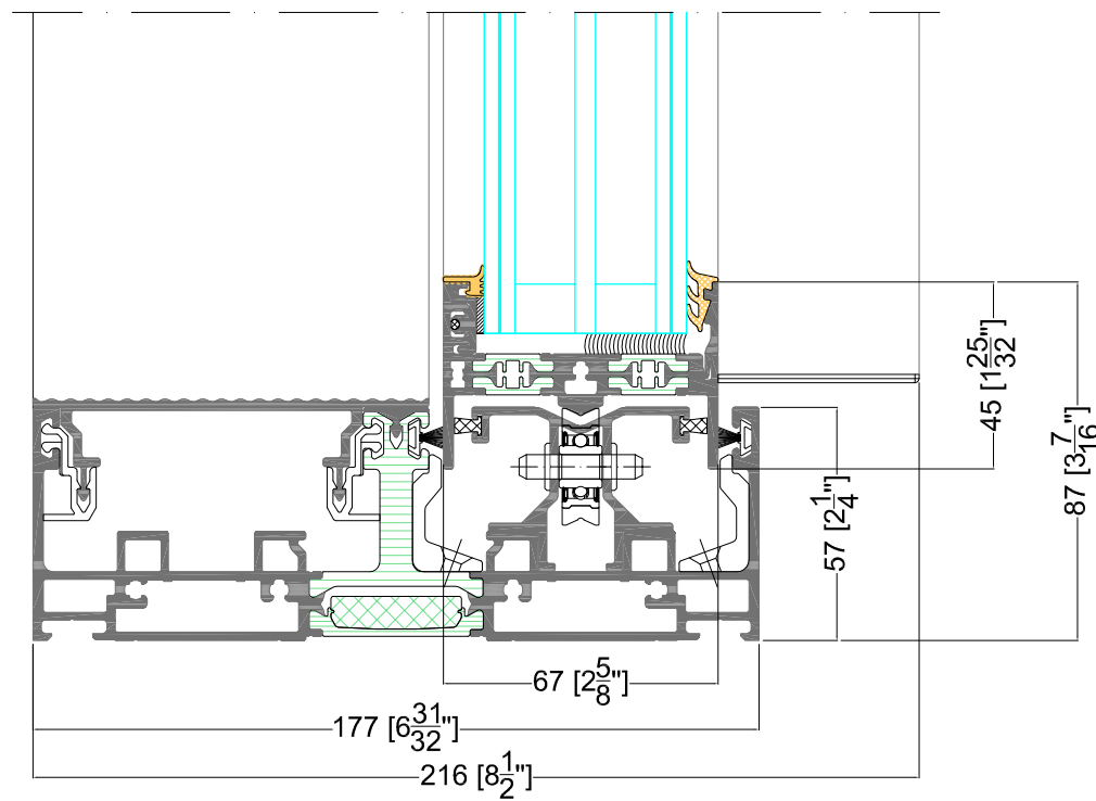
FLUSH TRACK - EXPOSED FRAME
