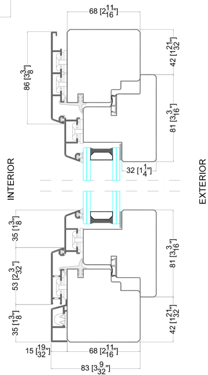
DETAIL 2
