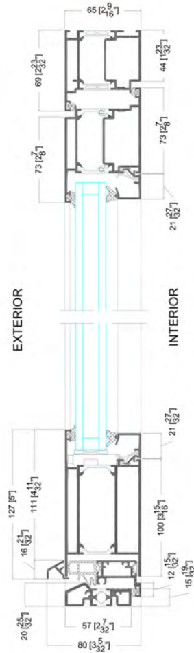
DETAIL 2
